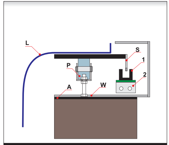
Fig. 17. Installation and positioning the encoder
